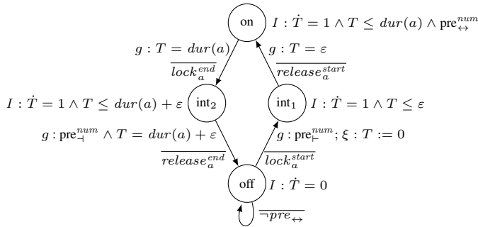
Figure 3: Structure of action automaton \mathcal{H}_a
