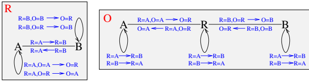
Figure 3: Atomic projections in (simplified) Gripper.
