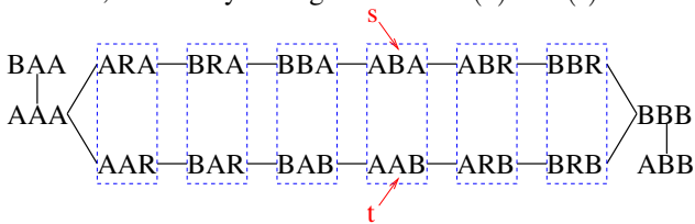
Figure 1: An abstraction of (simplified) Gripper.
