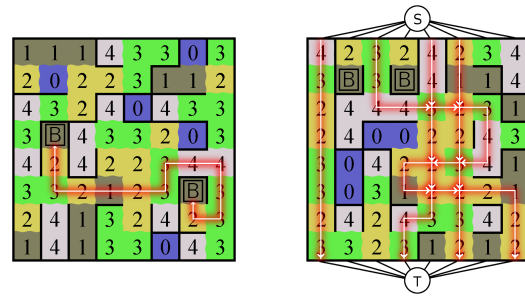
Figure 1: Diorama heightmaps generated by MONOSAT. Numbers correspond to elevations (bases are marked ‘B’), with impassable cliffs marked in black. On the left, a distance constraint between bases; on the right, a maximum s-t flow constraint between the top and bottom of the map.
