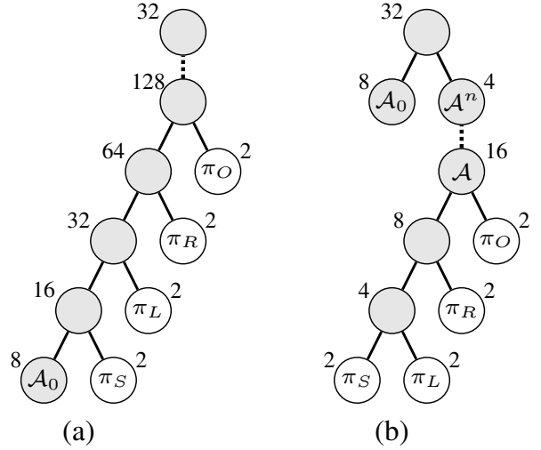
Figure 4: The merge-and-shrink trees of merging \mathcal{A}_0 with \pi_S, \pi_L, \pi_R, \pi_O linearly (a) and non-linearly (b). The sizes of the abstractions are marked beside the nodes. The dotted line indicates the operation that removes unnecessary states. Gray nodes are intermediate (non-atomic) abstractions.
