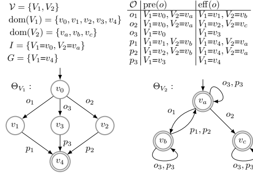
Figure 2: Example planning task with atomic factored LTS \langle \Theta_{V_1}, \Theta_{V_2} \rangle . All operators have a unit cost.
