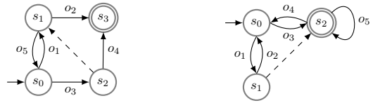
Figure 1: Examples of transition systems with redundant states. The dashed arrows show where to map redundant states.
