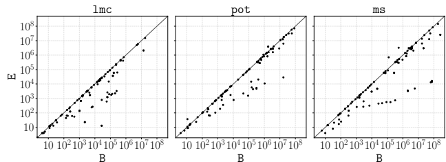
Figure 4: Number of expansions before the last f layer for tasks solved both with and without pruning using endomorphisms where at least one operator was pruned. B and E as in Table 2.
