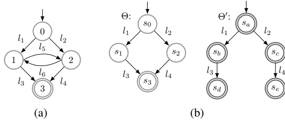
Figure 3: (a) an example of a symmetric LTS; (b) a factored LTS \langle \Theta, \Theta' \rangle .
