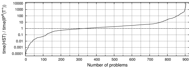
Figure 3: Computation of h^+ : Comparison of IP^e(T^+) and HST on delete-free, relaxed problems
