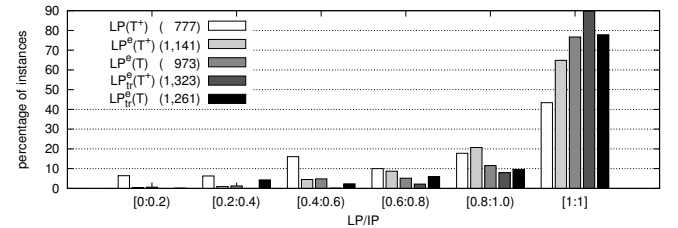
Figure 2: Ratio between the optimal costs of the IP’s and their LP relaxations, categorized into buckets. [x:y) = “% of instances where the LP/IP ratio is in the range [x:y)”.
