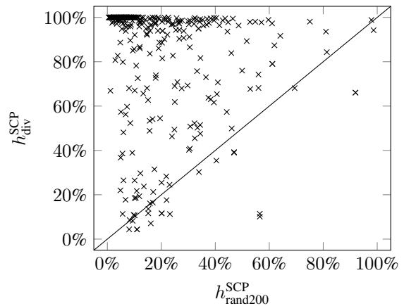
Figure 4: Percentage of probably useful orders for 200 random orders ( h_{\text{rand200}}^{\text{SCP}} ) and diverse orders ( h_{\text{div}}^{\text{SCP}} ). We exclude tasks for which any of the two heuristics uses fewer than 1000 expansions. Results are averaged over 10 runs.
