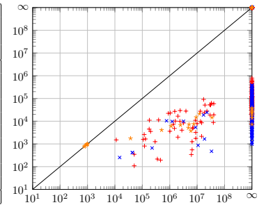
Figure 2: Empirical results. Left: Coverage. Best per-domain results highlighted in boldface. DFS-CL is our approach, \alpha = \infty with unlimited learning, \alpha = 1 without learning. Other abbreviations see text. For each domain, there are 30 or 5 base instances as specified (union of Nakhost et al.’s “small” and “large” test suites, for NoMystery and Rovers). For each base instance and value of W , the resource budget is set according to W . Right: Search space size for DFS-CL with learning ( \alpha = \infty , y -axis) vs. without learning ( \alpha = 1 , x -axis). “+” (red) NoMystery, “x” (blue) Rovers, “*” (orange) TPP, “∞”: out of time or memory.
